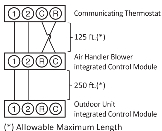
System Wiring
